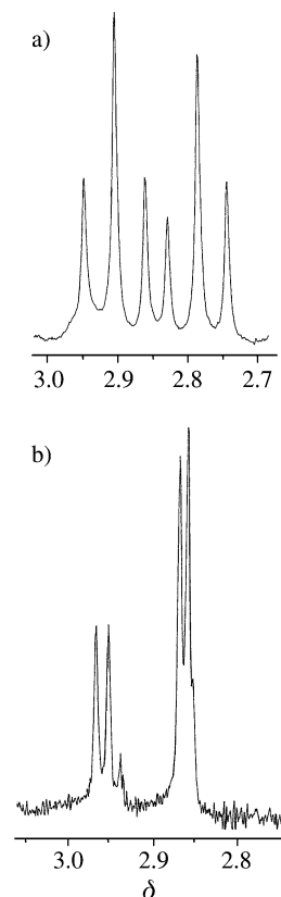
Fig. 1 Part of the 300 MHz ^1H NMR spectra of (a) L^{14} and (b) [L^{14} + H]^+ in CD_3CN (298 K).
